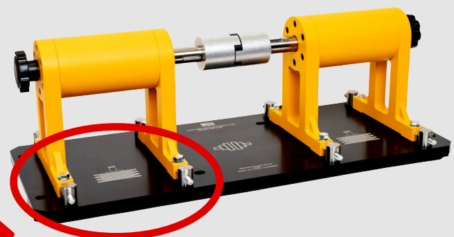
Reposition Jack Bolts for SHAFT ALIGNMENT
